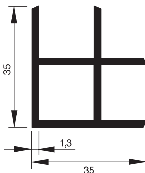
Art. P7302A-M6 argento € 9,50/mt. Art. P7302N-M6 nero € 11,25/mt. Art. P7302V-M6 bianco € 11,25/mt. Profilo 35x35mm, barre da 3/6 mt.
